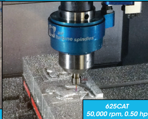
Hurco VM10i
