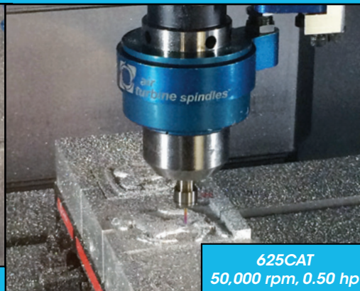
Hurco VM10i
